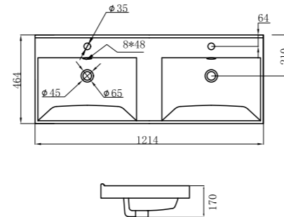
CABINET WASHBASIN Dimension: 1214*464*170mm
