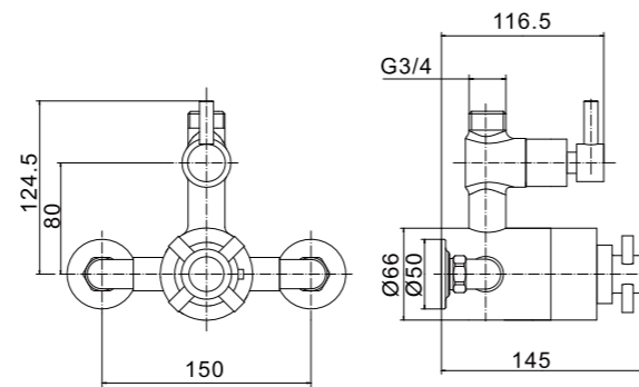
PT85710 Traditional exposed thermostatic shower valve
