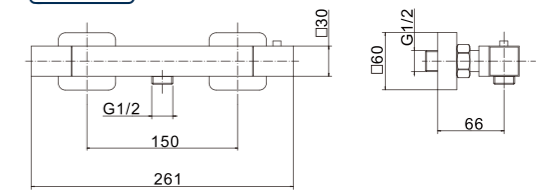
PT80814M Exposed thermostatic bar valve
