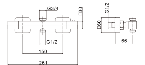
PT8089M Exposed thermostatic bar valve
