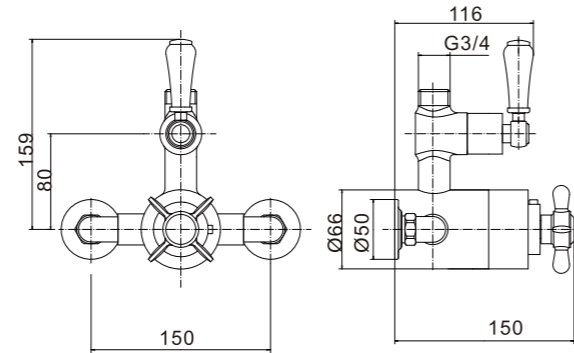
PT8573 Traditional exposed thermostatic shower valve
