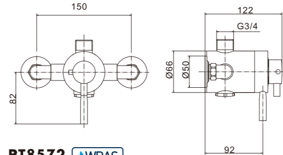
PT8572 Traditional exposed thermostatic shower valve
