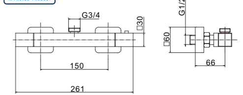
PT8087M Exposed thermostatic bar valve
