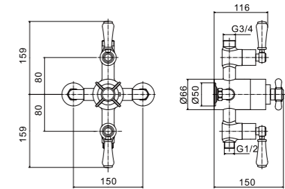
PT8577 Traditional exposed thermostatic shower valve
