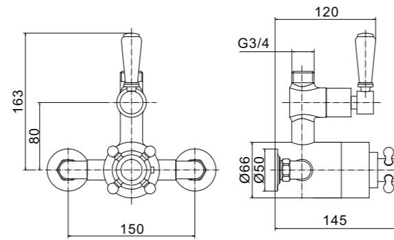
PT8578 Traditional exposed thermostatic shower valve
