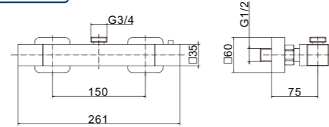
PT8087 Exposed thermostatic bar valve
