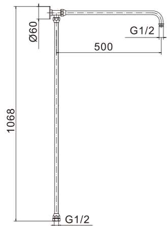
PS2010 Rigid riser kit
