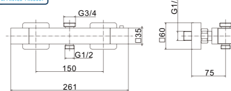
PT8089 Exposed thermostatic bar valve
