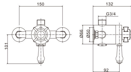
PT85713 Traditional exposed thermostatic shower valve
